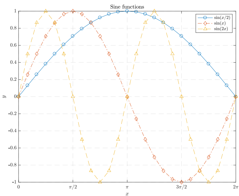
Figure 1: Sine functions
